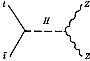
Fig. 2. Higgs exchange diagram for t\bar{t} \rightarrow ZZ .
