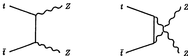
Fig. 1. Conventional diagrams for t\bar{t} \rightarrow ZZ .
