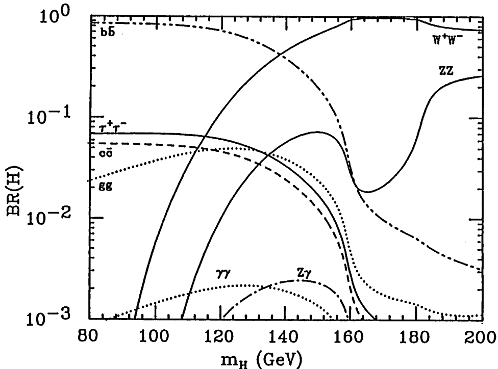
Fig. 4. Standard Higgs branching ratios in the “intermediate” region m_H = 80\text{--}200 GeV. m_t = 100 GeV assumed.
